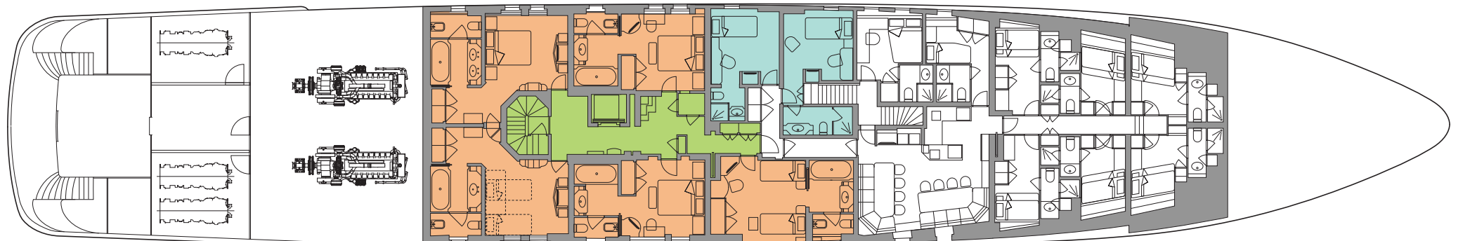
LOWER DECK
